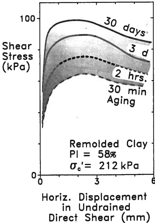
FIG. 13. Example of Laboratory Increase in Undrained Strength of Clay due to Aging in Secondary Compression
