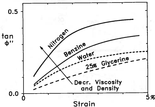
FIG. 35. Comparative Mobilized \tan \phi'' Behavior from Same Tests as in Fig. 34
