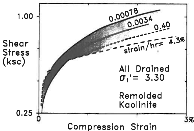
FIG. 31. Comparative IDS Compression Tests using Different Rates of Strain
