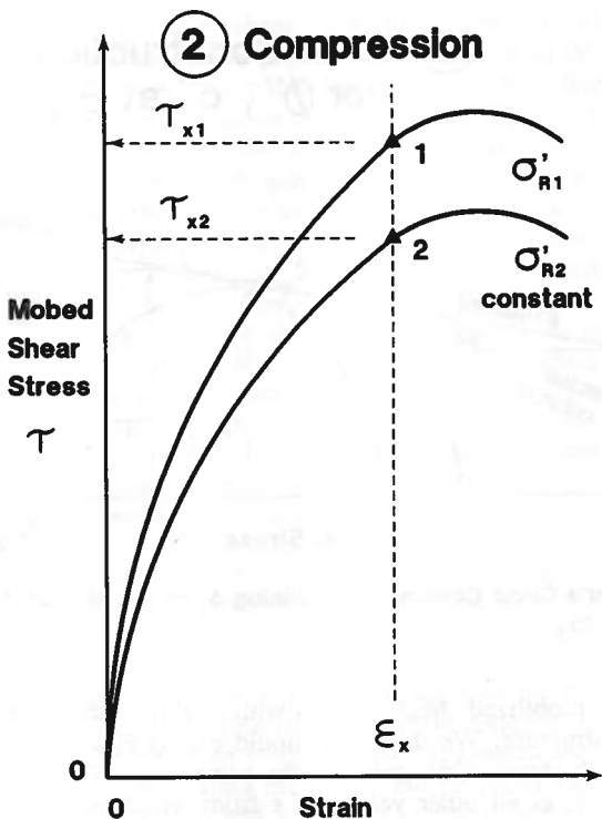
FIG. 21. Comparative Compression Tests having Same Soil Structure at Every Magnitude of Strain
