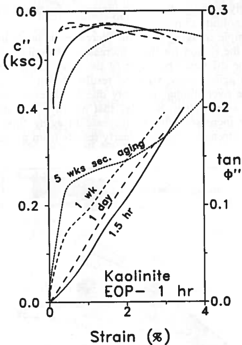
FIG. 30. Comparative IDS-Test c'' and \tan \phi'' Components after Various Times in Secondary Compression Aging
