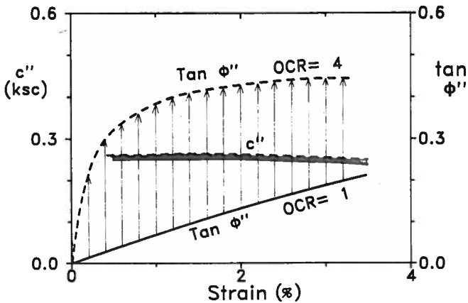
FIG. 37. Comparative IDS-Test c'' and \tan \phi'' Mobilization for Same OCR of 1 and 4 Tests in Fig. 36
