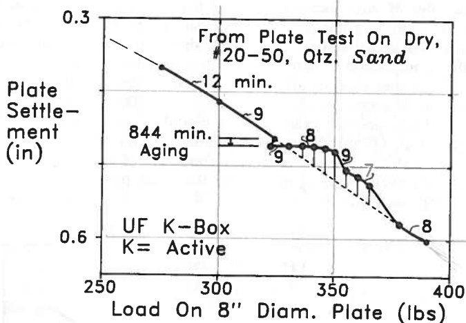
FIG. 6. Aging-Preconsolidation Effect Demonstrated for Plate Load Test in SC-UF Lateral Stress Box
