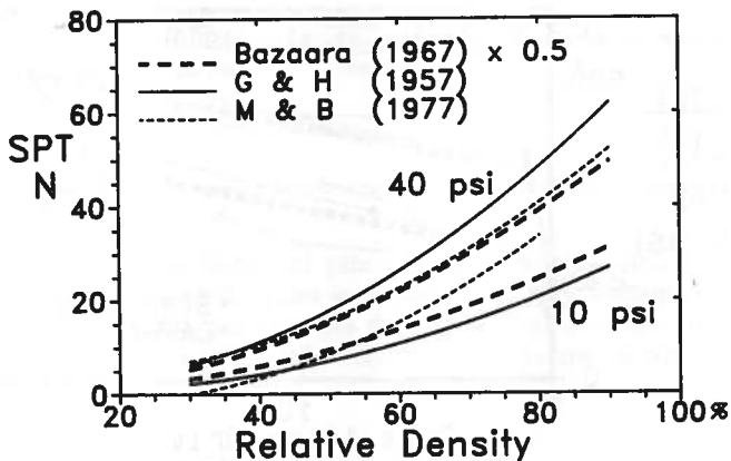
FIG. 15. Well-Known Field and Lab Chamber Correlations between N and Relative Density Match Better after Aging Correction
