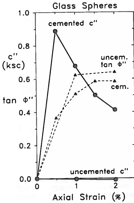
FIG. 25. \phi'' and c'' Component Separation for Tests in Fig. 24
