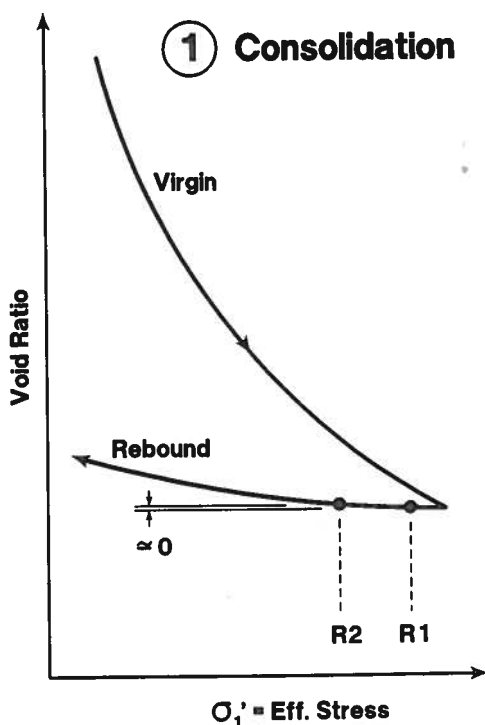
FIG. 20. Selection of Two Points In Soil's Stress History for Nearly Constant Structure at Different Effective Stress
