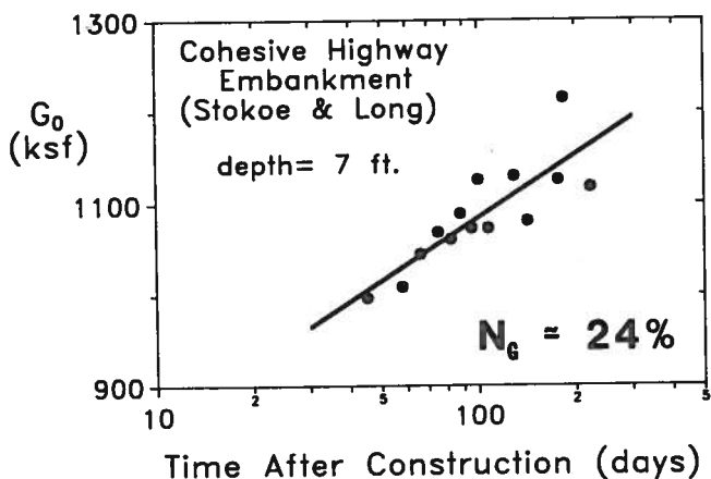
FIG. 8. Example of Small Strain Shear Modulus Increase In Field
