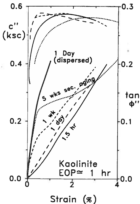
FIG. 38. Comparing \tan \phi'' Mobilization of Dispersed Kalonite with that of Relatively Undispersed Kalonite Subjected to Various Times in Secondary Compression Aging
