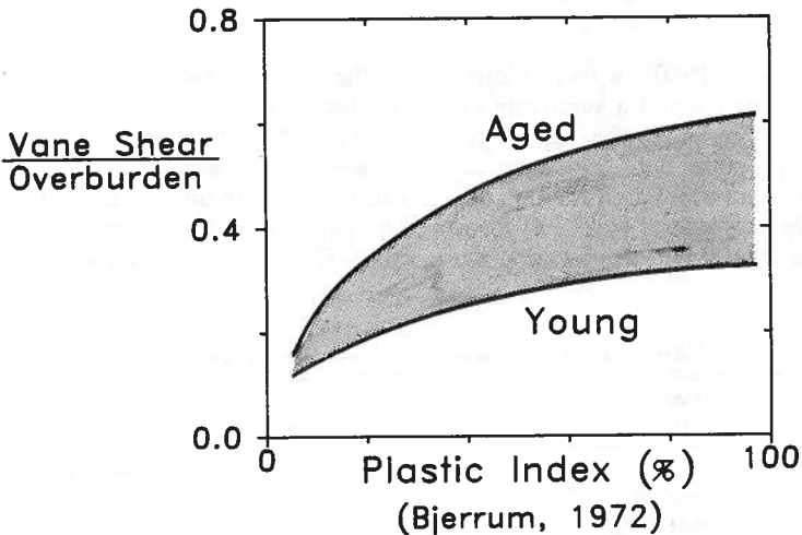
FIG. 12. Geologic Aging Increases Normalized Field Vane Shear Strength in Near-Normally Consolidated Clays
