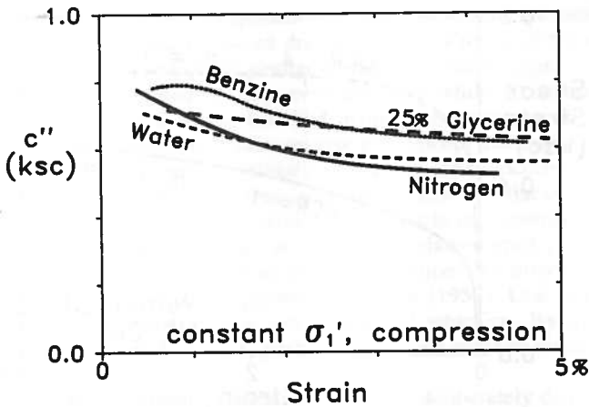
FIG. 34. Comparative c'' Mobilization Behavior from Compression Tests using Kalonite Powder Saturated with Different Pore Fluids
