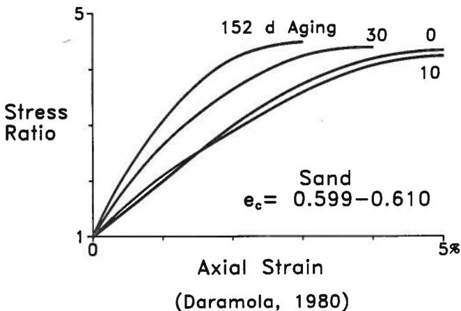
FIG. 10. Laboratory Example of Modulus of Sand Increasing with Secondary Compression Aging
