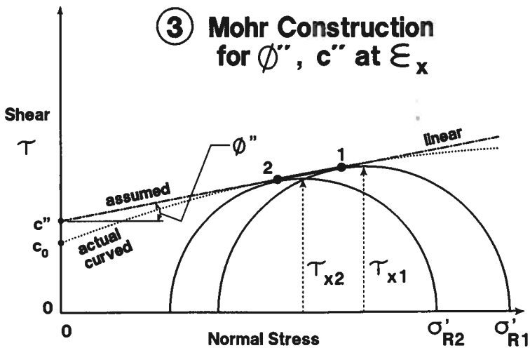
FIG. 22. Mohr's Circle Construction Defining \phi'' and c'' at Each Strain in Tests Shown in Fig. 21
