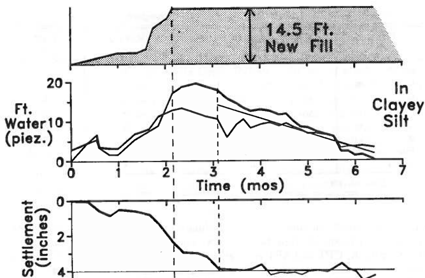
FIG. 19. Field Example Showing Pore-Pressure Dissipation with Time without Matching Consolidation Settlement
