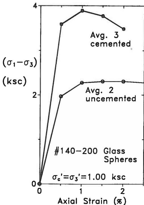
FIG. 24. Comparative IDS Compression Test Results using Glass Beads with and without Hydrocal Cementation
