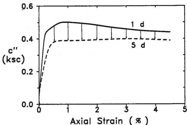
FIG. 28. Comparative c'' Components from Fig. 27 Tests
