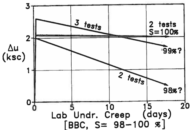
FIG. 18. Laboratory Example of Pore-Pressure Dissipation with Time under Undrained Creep Conditions
