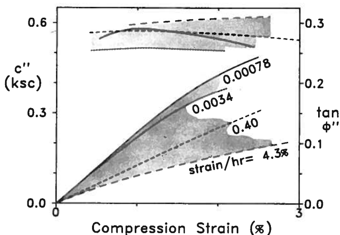
FIG. 32. Comparative c'' and \tan \phi'' Component Separations from Fig. 31 Tests
