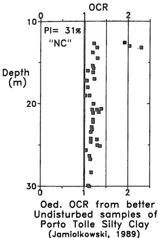
FIG. 4. Subsequent, Superior Data Showing Aging-Preconsolidation Effect in Same, Supposedly Normally Consolidated Clay
