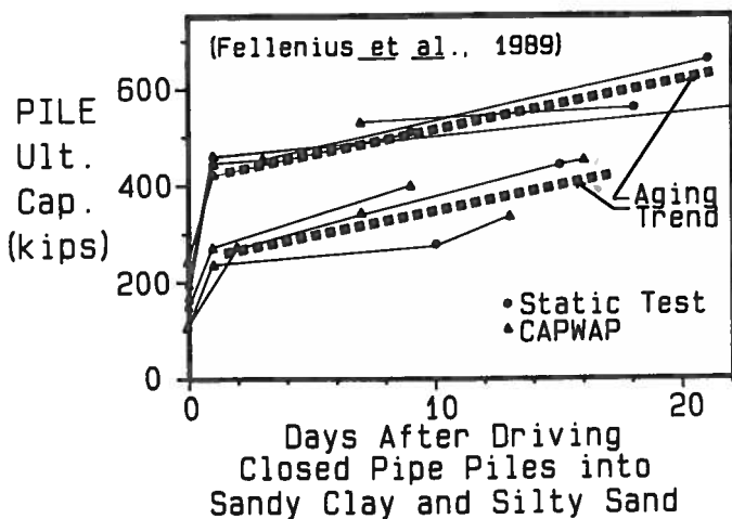
FIG. 17. Project Compression Pile Load Tests Show Capacity Gain with Time after Probable Full Excess Pore-Pressure Dissipation
