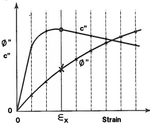
FIG. 23. \phi'' and c'' Plotted as Functions of Strain, Based on Fig. 21 Tests and Fig. 22 Constructions
