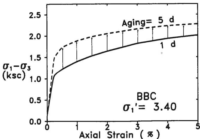
FIG. 27. Average Laboratory Compression Tests after One Day and Five Days of Secondary Compression Aging
