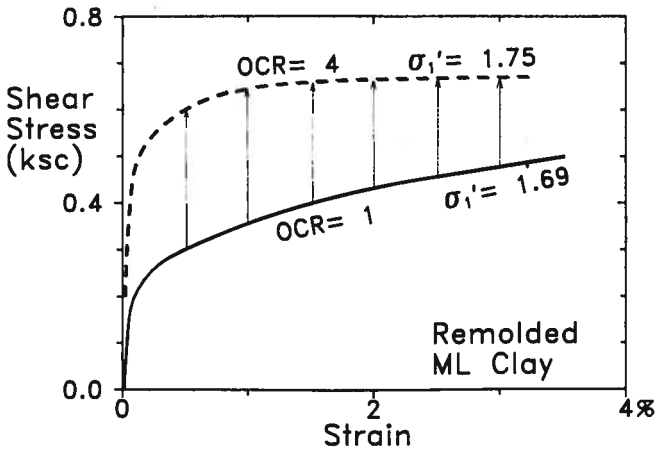
FIG. 36. Comparative Compression Tests from Duplicate Specimens of Same Clay Consolidated to OCR Ratios of 1 and 4
