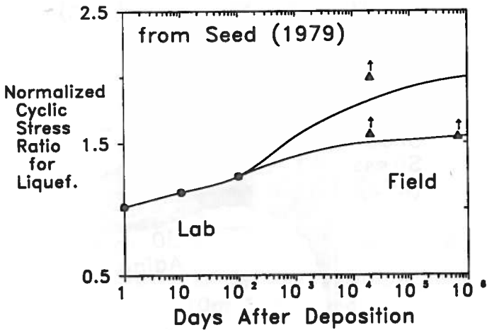
FIG. 11. Laboratory and Field Data Illustrating Increased Resistance to Liquefaction with Aging
