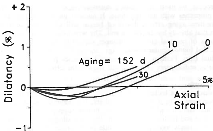
FIG. 33. Comparative Aging-Dilatancy Behavior for Sand Compression Tests in Fig. 10
