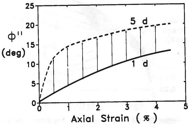
FIG. 29. Comparative \phi'' Components from Fig. 27 Tests
