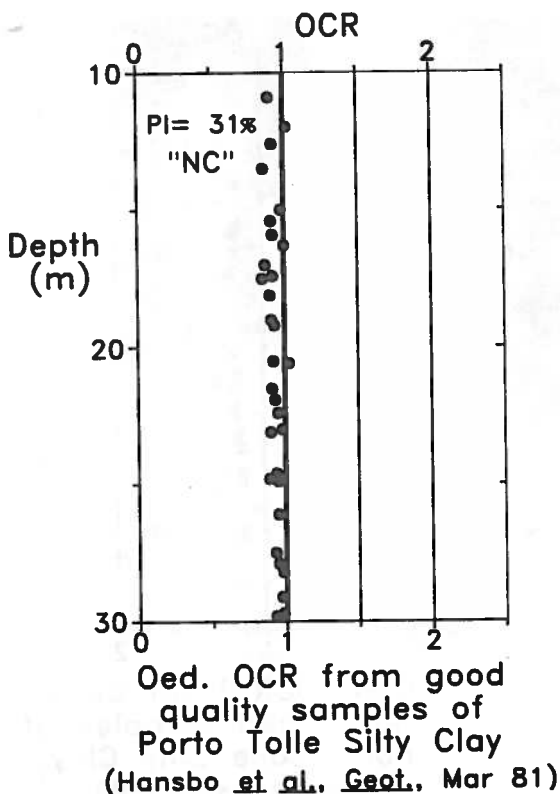
FIG. 3. Example of High-Quality Laboratory Data Mistakenly Denoting Clay as Truly Normally Consolidated
