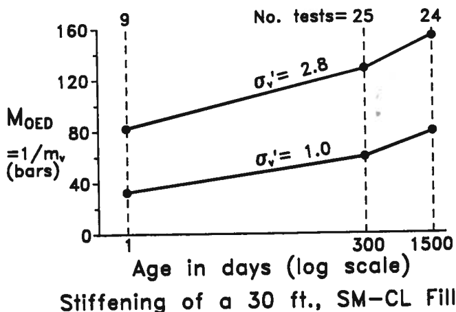
FIG. 7. Example of Aging Increasing Oedometer Modulus In Compacted, Cohesive Fill
