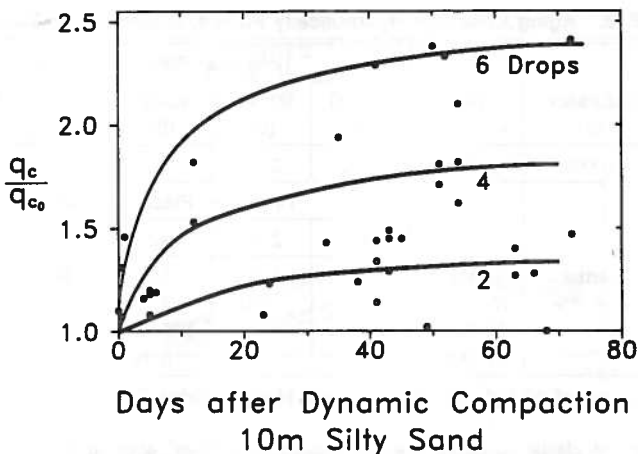
FIG. 14. Normalized Increase in Static-Cone Bearing Capacity after Dynamic Compaction
