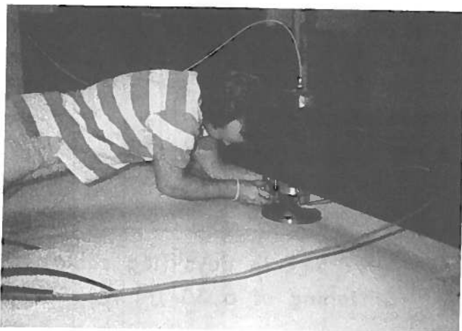
FIG. 5. Final Stages of Setting Up Fig. 6 Plate Load Test in Schmertmann & Crapps, Inc.—University of Florida Lateral Stress Sand Box
