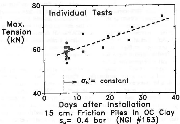
FIG. 16. Research Pile Tension Tests Show Pile Capacity Gain during Aging under Constant Effective Stress Conditions
